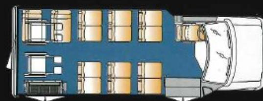
12 Passenger 2 Wheelchair 4 Passenger Foldaway Seats Plus Driver
